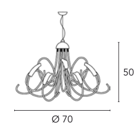
Chic 2010/S5L 5 x max 40W G9 230V CE V
